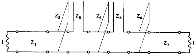
Figure 2 Seven-section filter containing unit elements and stubs. All sections are quarter-wave at 2.175 GHz
